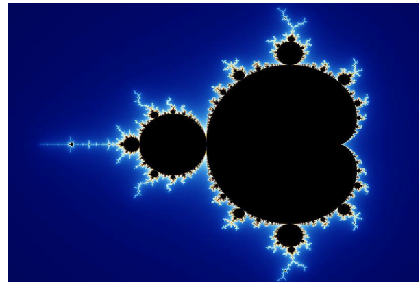
Mandelbrot Set
